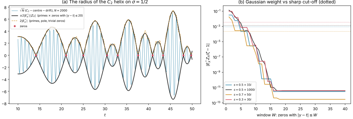
FIGURE 4. The factorization \zeta = E_X^* Z_X seen by C_2 , Gaussian weight of standard deviation 0.4, X = 1000.5 . (a) C_2(n, \frac{1}{2} + it) minus its centre 1/(\frac{1}{4} + t^2) and its Bernoulli terms, multiplied by \sqrt{n} , for n = 2000 , against \pm 2|E_X^*||Z_X| with the zeros |\gamma - t| \leq 20 and against the prime factor 2|E_X^*| alone; dots: zeros. (b) The relative error of E_X^* Z_X against the window W of zeros used, at four points (Table 10); dotted: the sharp cut-off at x = 1000.5 with the 1517 zeros below height 2000.
