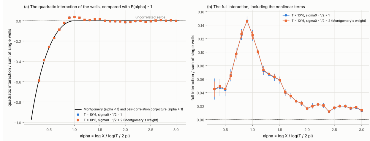
FIGURE 1. The interaction of the wells at height T = 10^6 , X = (T/2\pi)^\alpha , averaged over 200 centres, relative to the sum of the single wells. (a) The quadratic part against -\frac{\pi}{\kappa_1}(1 - \alpha + \alpha \log \alpha) for \alpha < 1 (Montgomery's theorem under RH, with the contribution of \beta \geq 1 set to 0) and 0 for \alpha > 1 (pair-correlation conjecture). (b) The full interaction.
