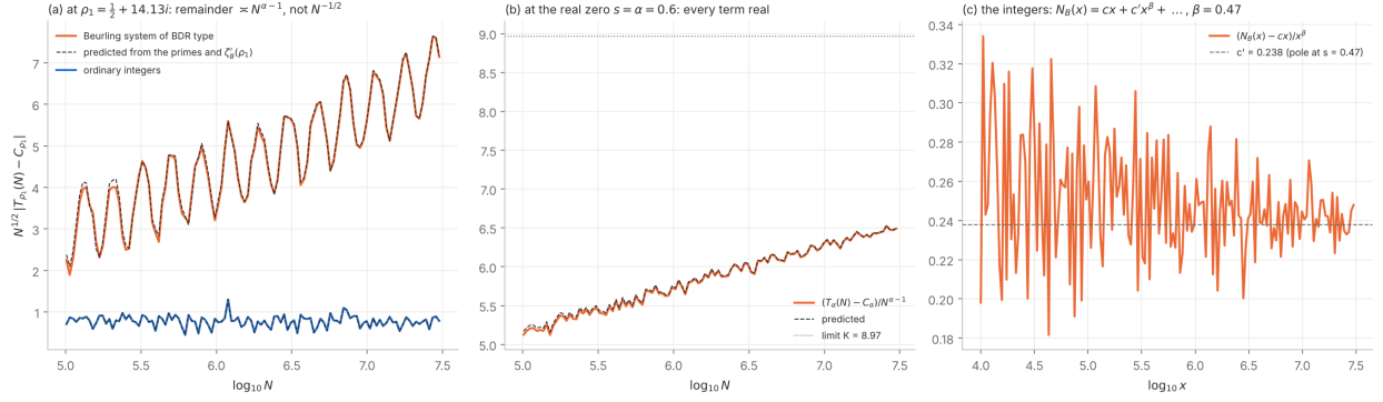
FIGURE 7. A Beurling system with the zeros of \zeta and a real zero at \alpha = 0.6 ( \beta = 0.47 ). (a) N^{1/2}|T_{\rho_1}(N) - C_{\rho_1}| for the system and for the integers, with the prediction of Proposition 51(ii) (dashed). (b) At the real zero: (T_{\alpha}^B(N) - C_{\alpha})/N^{\alpha-1} , the prediction and its limit K . (c) (N_B(x) - cx)/x^{\beta} and c' .
