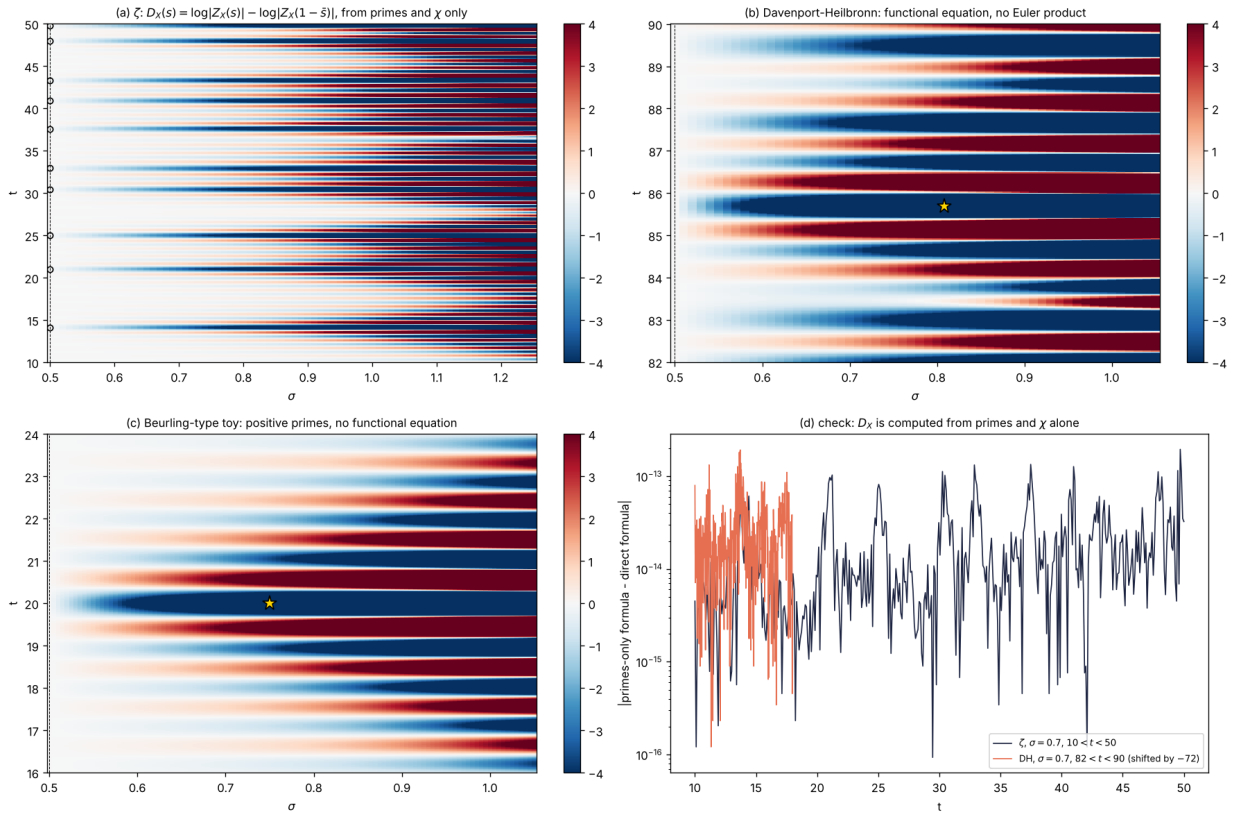
FIGURE 8. The reflection asymmetry D_X(s) , X = 10^3 , Gaussian weight of standard deviation 0.4. (a) \zeta , from the primes and \chi only; circles: zeros. (b) The Davenport–Heilbronn function near its off-line zero (star), from its coefficients and its \chi . (c) A Beurling-type toy with the nonnegative prime measure (1 - 2 \operatorname{Re} x^{\rho_B - 1}) dx / \log x on [16, \infty) , \rho_B = 0.75 + 20i (star), and no functional equation, from its two zeros. (d) Difference between the primes-only formula and the direct one on \sigma = 0.7 .
