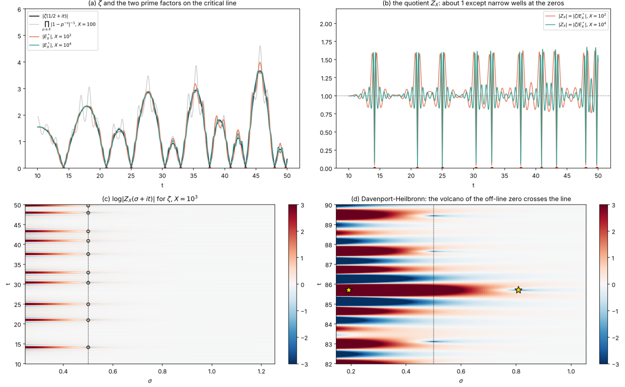
FIGURE 3. (a) |\zeta(\frac{1}{2} + it)| , the truncated Euler product \prod_{p \leq X} |1 - p^{-s}|^{-1} with X = 100 , and |E_X^*| for X = 10^2, 10^4 . (b) |Z_X| on the line: wells with the profile e^{\text{Ci}(|v|)} . (c) \log |Z_X(\sigma + it)| for \zeta , X = 10^3 : craters on the line, volcanoes to the left. (d) The same for the Davenport–Heilbronn function near its off-line zero 0.8085 + 85.699i : its volcano crosses the line.
