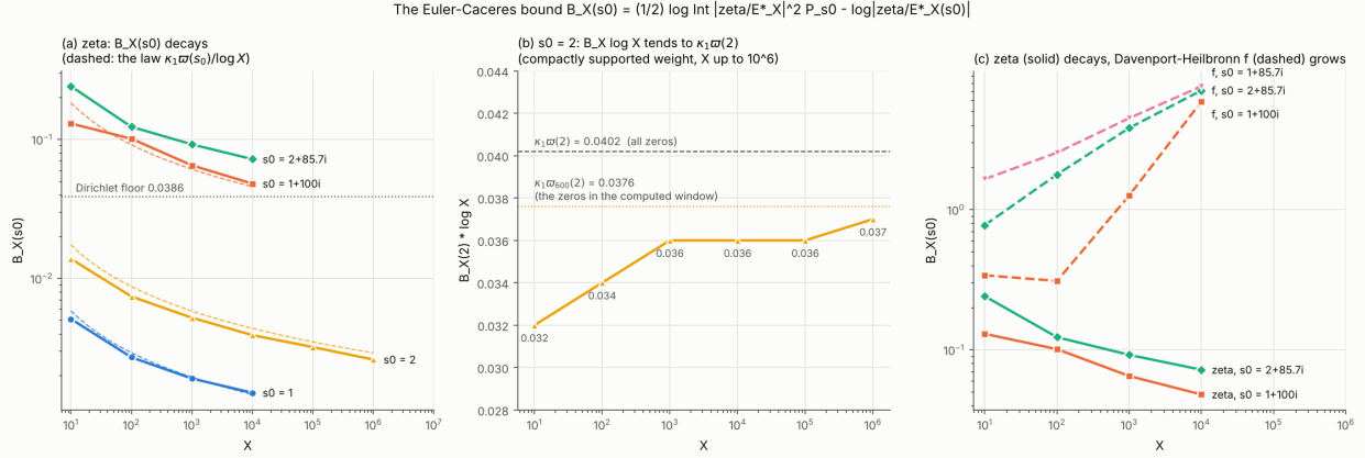
FIGURE 2. The Euler–Caceres bound (data of Table 7 and of the window-600 computation above). (a) B_X(s_0) for \zeta at four centres, with \kappa_1 \varpi(s_0)/\log X (dashed) and the floor 0.0386 of Dirichlet mollifiers (dotted). (b) (\log X)B_X(2) , window |t| \leq 600 , against \kappa_1 \varpi(2) = 0.0402 and \kappa_1 \varpi_{600}(2) . (c) \zeta (solid) against the Davenport–Heilbronn function (dashed). Panels (a) and (c) use a Gaussian weight g_0 of standard deviation 0.4, with the prime sum truncated at 4.5 standard deviations, on |t - t_0| \leq 300 ( |t| \leq 2000 at s_0 = 1 ).
