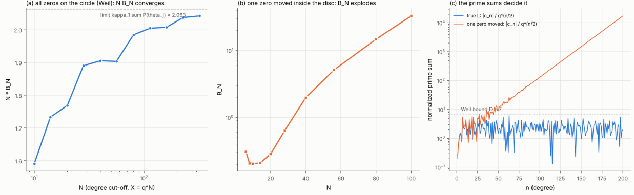
FIGURE 6. The Euler–Caceres bound over \mathbb{F}_3[T] , \deg L = 7 . (a) NB_N for the true L -function (all zeros on the circle, by Weil’s theorem). (b) B_N with one zero moved into the disc. (c) The normalized prime sums |c_n|q^{-n/2} : bounded by D for the true L , geometrically growing for the perturbed one.
