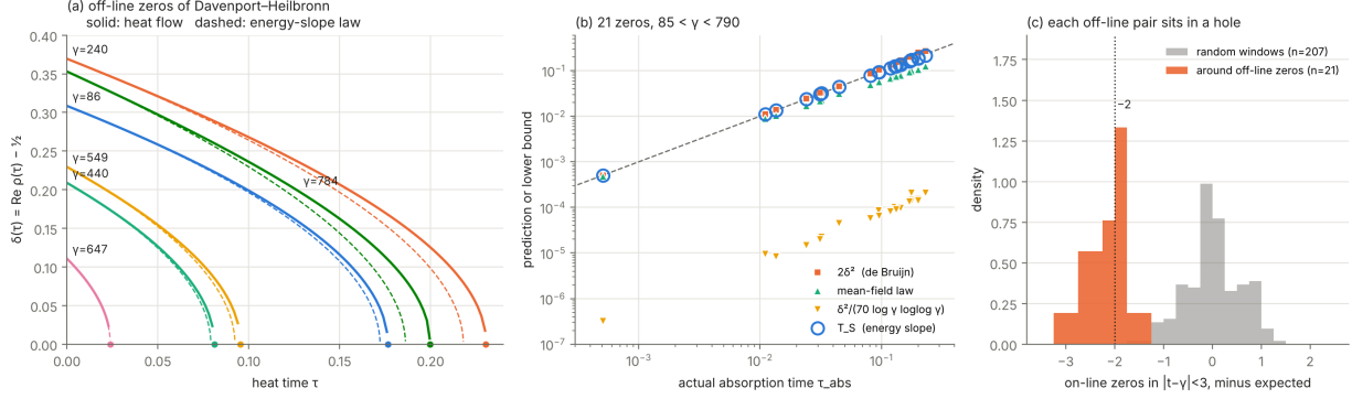
Figure 4: The Davenport–Heilbronn test. (a) Six of the 21 off-line zeros under the heat flow (solid) and the energy-slope law with S_{\text{rest}} frozen at \tau = 0 (dashed); dots mark \tau_{\text{abs}} . (b) Predictions and bounds against the measured absorption time; the dashed line is equality. (c) Number of zeros on the line within 3 units of each off-line zero, minus the expected number, against random windows.
