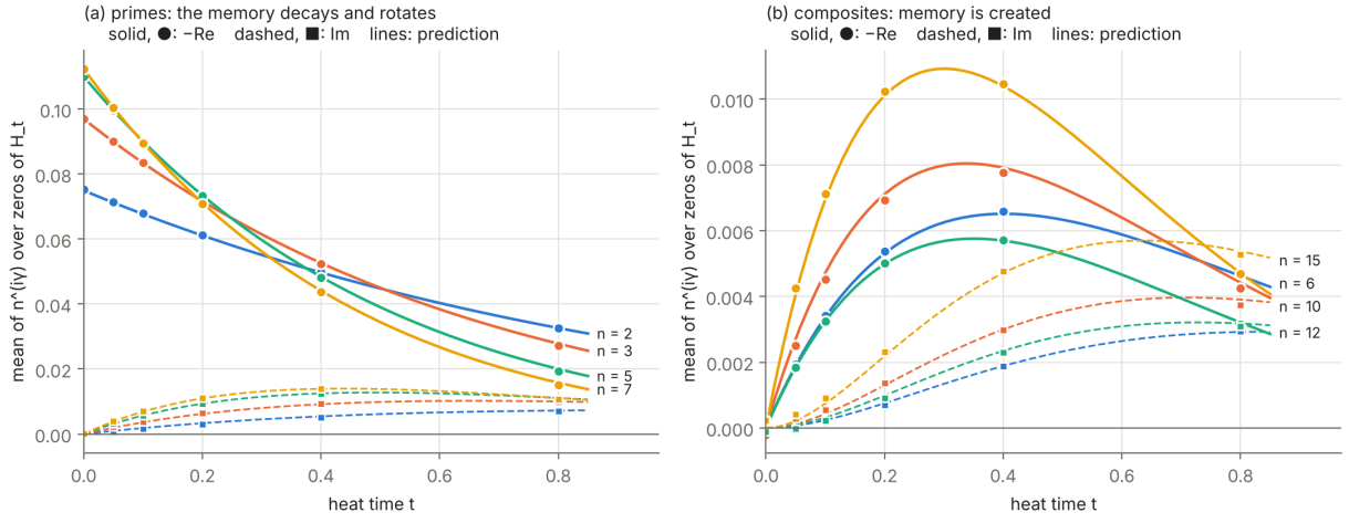
Figure 5: Arithmetic memory of the zeros under the heat flow. (a) Primes: -\text{Re} (solid, dots) and \text{Im} (dashed, squares) of \langle p^{i\gamma_k(t)} \rangle , measured, and Conjecture 10.2 (lines). (b) The same for the composites 6, 10, 12, 15, whose memory is created by the flow.
