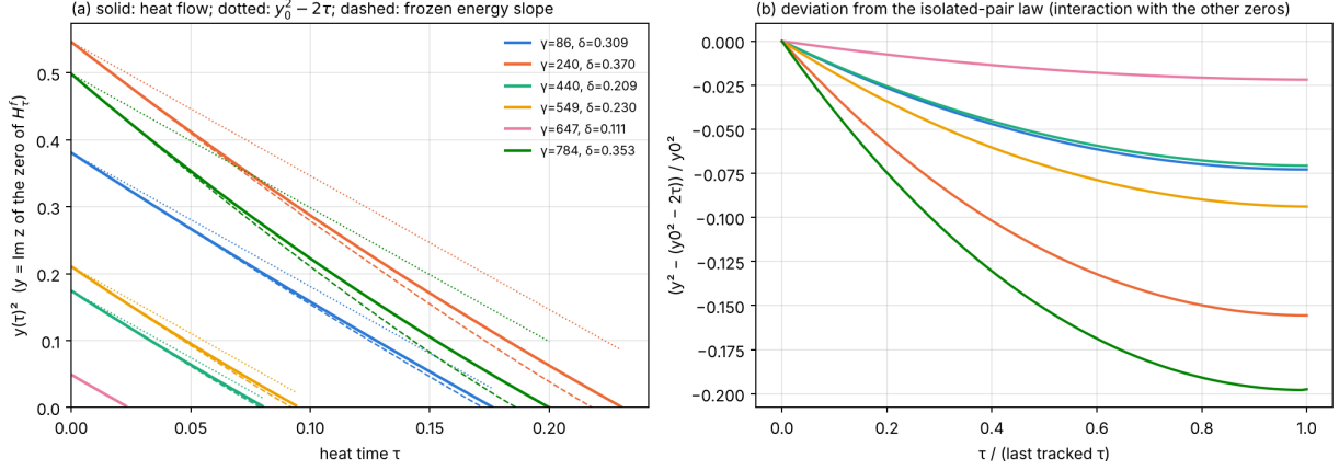
Figure 3: y(\tau)^2 for six of the off-line zeros of the Davenport–Heilbronn function under the heat flow, with y = \text{Im } z of the corresponding zero of H_\tau^f ( y_0 = 2\delta ). (a) The flow (solid), the isolated-pair law y^2 = y_0^2 - 2\tau (dotted) and the frozen energy-slope law \partial_\tau y = -1/y - S_{\text{rest}}(0) (dashed). (b) The relative deviation from the isolated-pair law, which measures the interaction with the other zeros.
