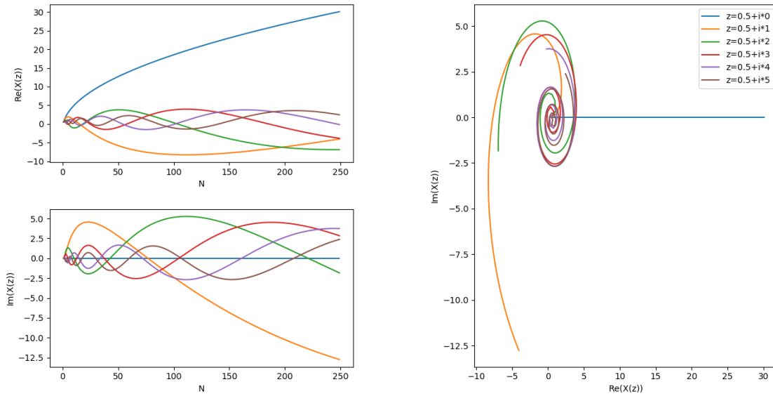
Figure. 7: X(z, n)
