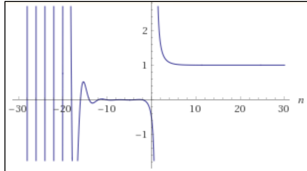
Figure. 1. Riemann Zeta function in R
