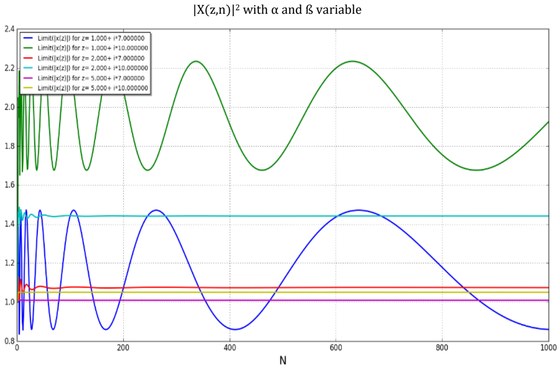
Figure. 20. |X(z, n)|^2 converges when n \rightarrow \infty and \alpha > 1
