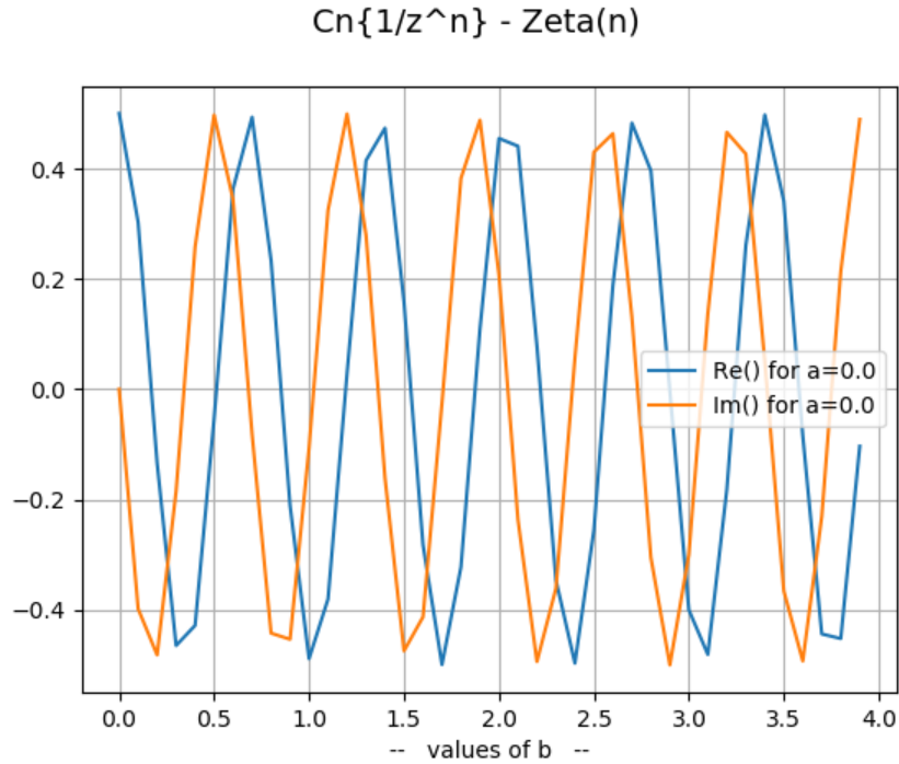
Figure. 4b. Where a=Re(z) and b=Im(z)
