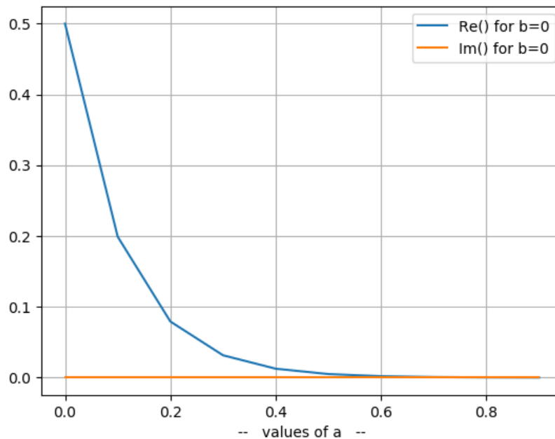
Figure. 4a. Where a=\text{Re}(z) and b=\text{Im}(z)
