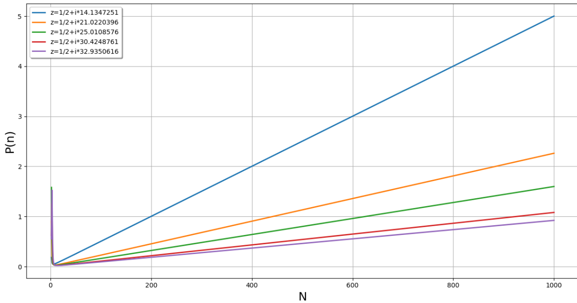
Figure. 26. Straight Lines P(n)
