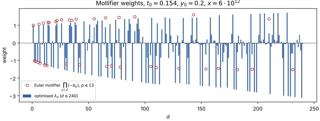
Figure 1: Optimised weights ( t_0 = 0.154 , d \leq 240 ) compared with Polymath's Euler mollifier on the primes up to 13, whose coefficients are \prod_{p|d} (-b_p) . The optimised mollifier uses every prime up to 240, with \lambda_p \approx -b_p , damps the squarefree composite terms, and gives some weight to prime powers (script weights_fig.py ).
