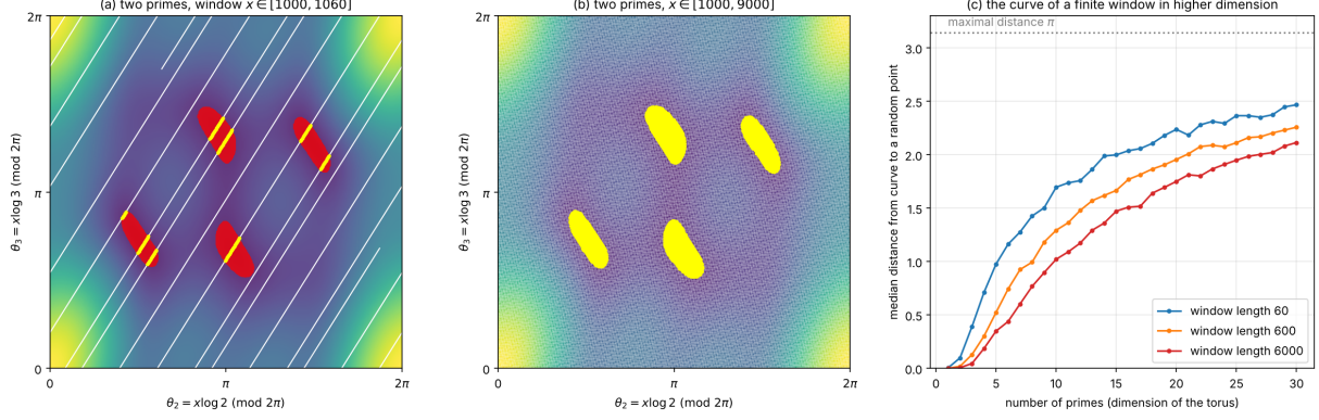
Figure 3: Phase torus versus the actual curve x \mapsto (x \log p \pmod{2\pi})_p . (a), (b): the Dirichlet polynomial \sum n^{-0.55} e^{-i\phi_n} over n \in \{1, 2, 3, 4, 6, 8, 9, 12\} , with \phi_n = v_2(n)\theta_2 + v_3(n)\theta_3 ; red: |\cdot| < 0.25 ; white: the curve; yellow: points of the curve in the red region. (c): median over 40 random target points of the sup-norm distance to the curve for x \in [10^4, 10^4 + L] , using the first d primes. Illustration only; no part of the proof depends on this figure.
