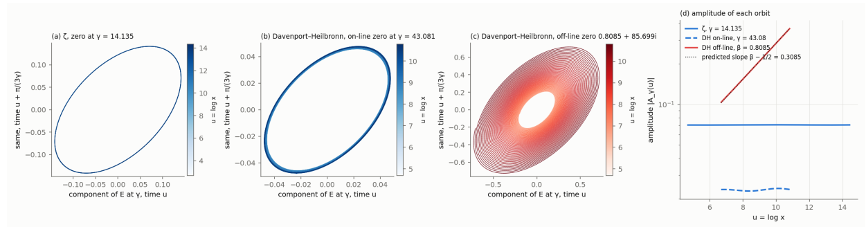
Figure 2: Orbits of the component at frequency \gamma of the normalised prime error E(u) , u = \log x , plotted against the same component at the delay \pi/(3\gamma) . (a) \zeta , \gamma = 14.135 . (b) Davenport–Heilbronn, on-line zero \gamma = 43.081 . (c) Davenport–Heilbronn, off-line zero 0.8085 + 85.699i . (d) Amplitudes, with the predicted slope \beta - \frac{1}{2} . Illustration only; no part of the proof depends on this figure.
