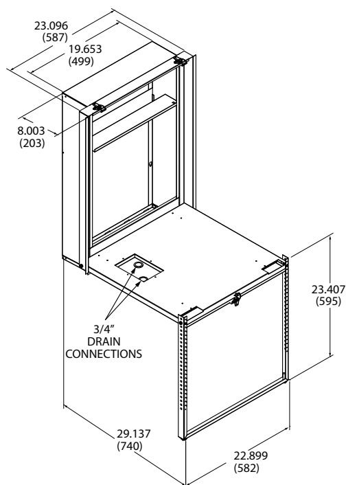
Wall Plenum Assembly Dimensions:
