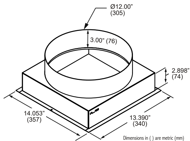
Discharge Plenum Dimensions (18kBTU and 24kBTU Units):
