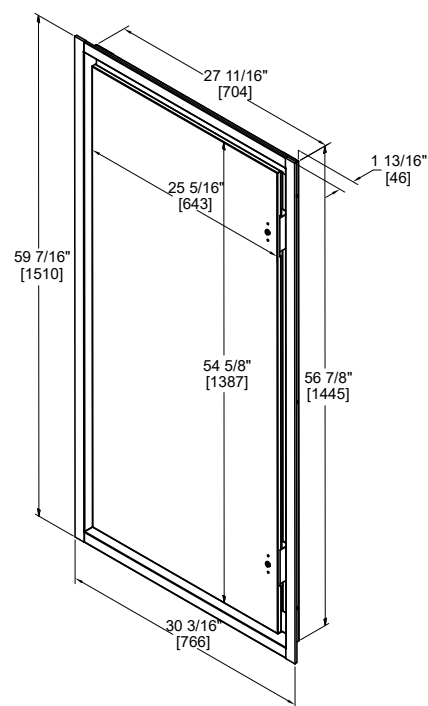
Hinged Access Panel Assembly Dimensions (All Units):
