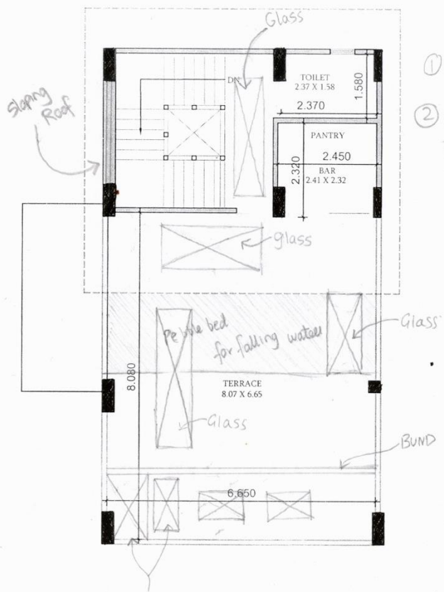
Glass TERRACE FLOOR PLAN
