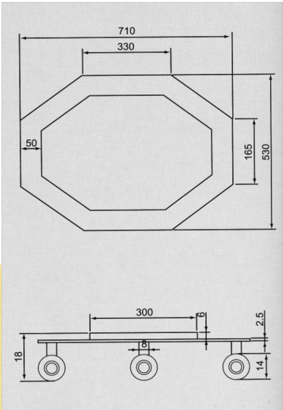
Plastic Tank with Wheels Material: PE Color: Blue Dimension: L800 x W650 x H700mm Volume: 210L
