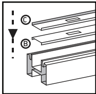
B. Snap Baluster Spacer into Bottom Rail. C. Place inverted Baluster Spacer on top of first Baluster Spacer.
