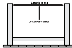
Length of rail \div 4.5 = balusters If number is odd: balusters will be centered If number is even: balusters will be offset 2 1/4" from center.
