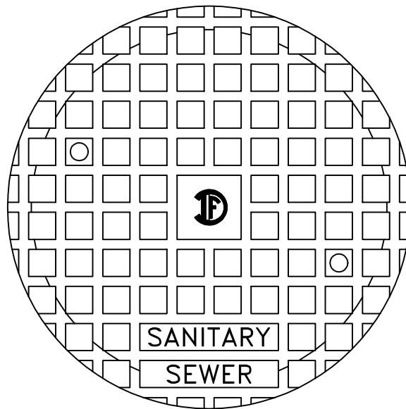
PLAN - COVER
