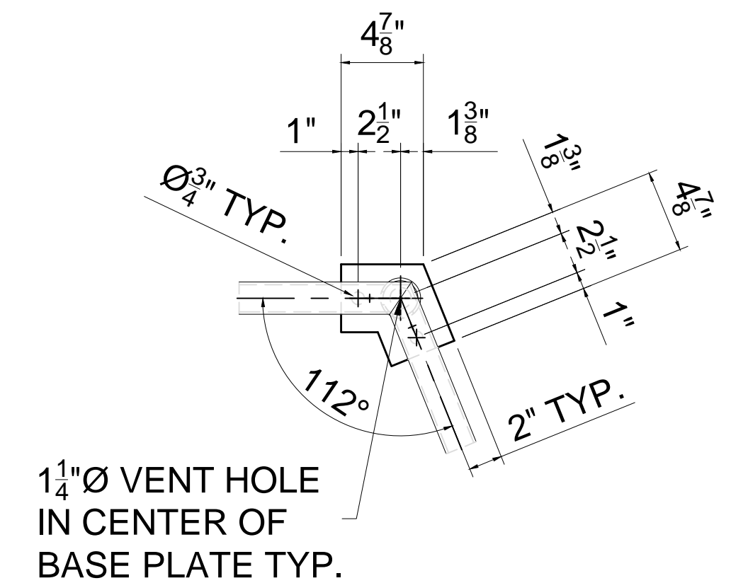
DETAIL C SHAPED BASE PLATE ASSEMBLY P5 - PLATE 1/2" X 4" X 4 7/8" TYP. @ L/H & R/H POSTS
