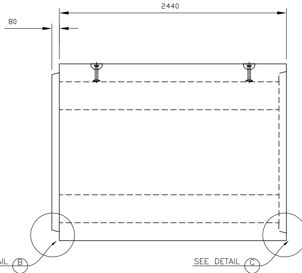
BOX SIDE ELEVATION SECTION-VIEW
