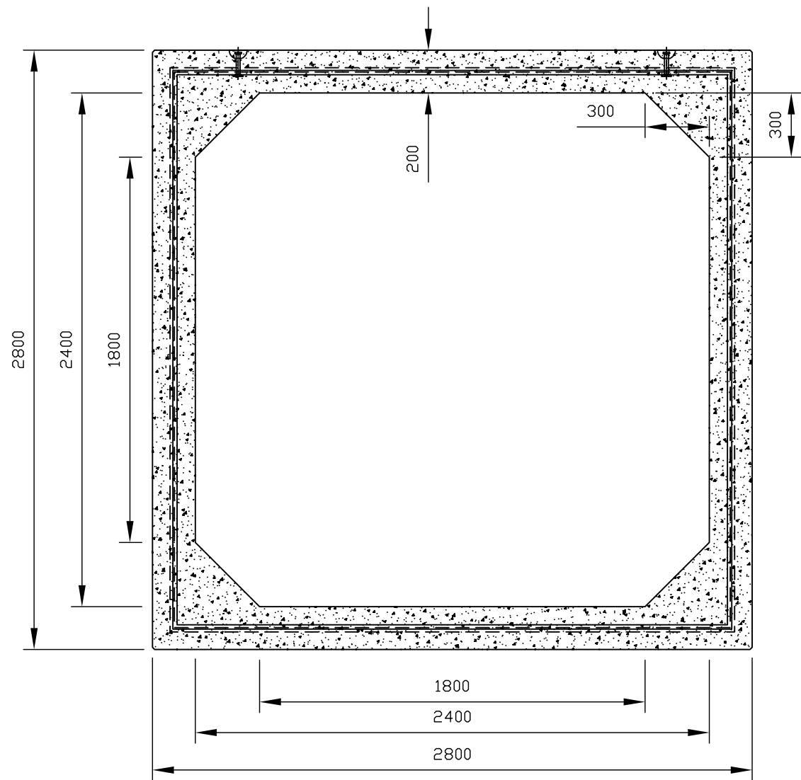
BOX CULVERT PLAN VIEW
