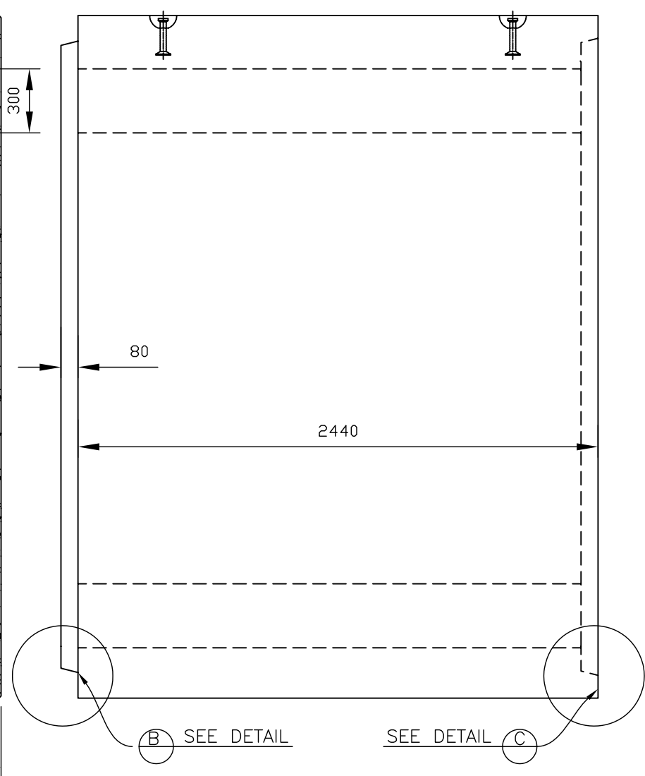
BOX SIDE ELEVATION SECTION-VIEW
