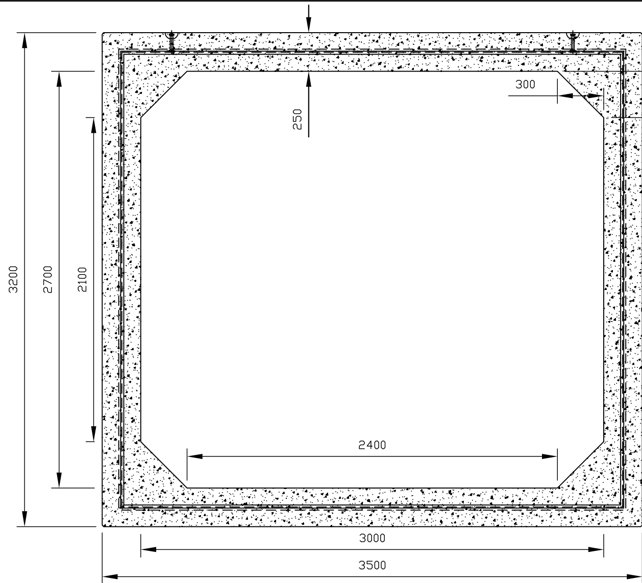
BOX CULVERT PLAN VIEW
