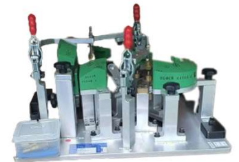
C/F Gauge
