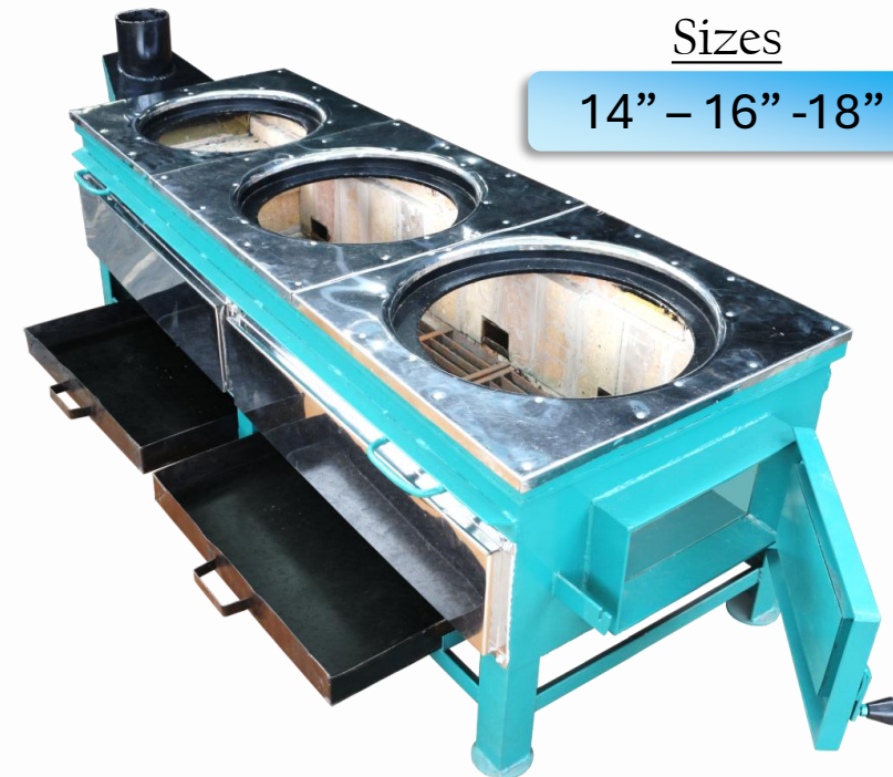
Triple Stove
