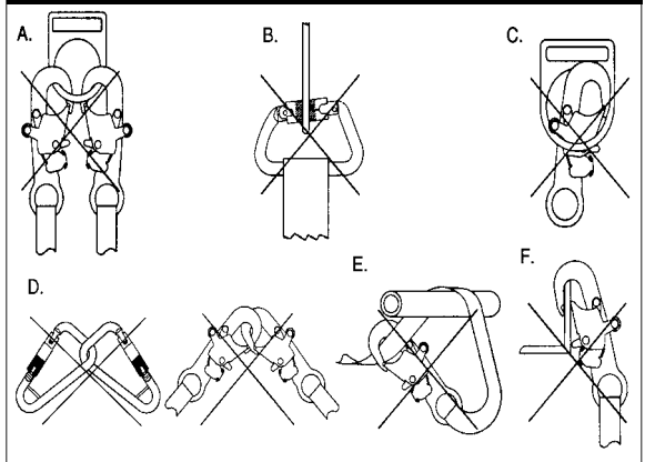
FIGURE 5 - INAPPROPRIATE CONNECTIONS
