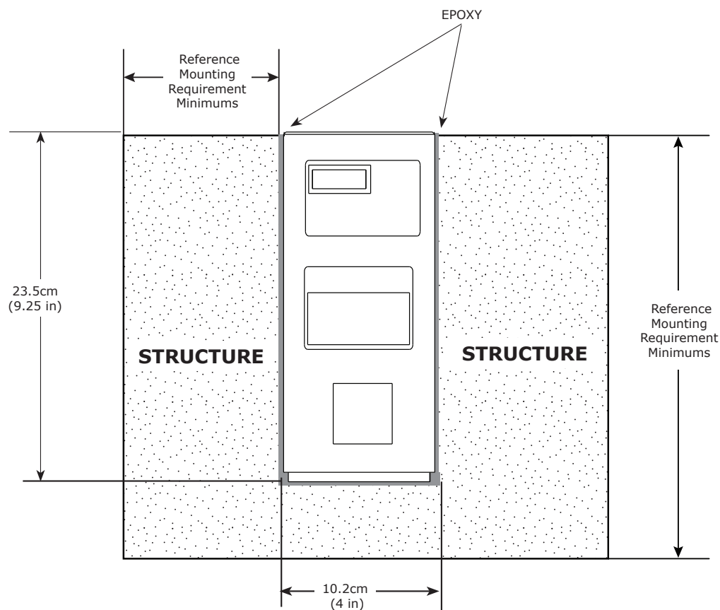
Figure 3 – Installing into Existing Concrete Method
