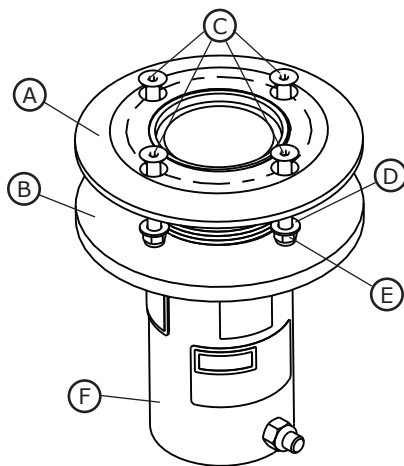
Figure 3 – Deck Mounted Davit Base Installation
