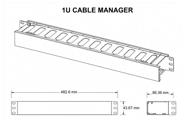
1U rack-mount cable manager with removable front cover
