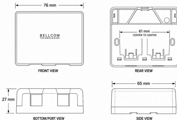
Bellcom 2-Port Surface Mount Box - Dimension Diagram
