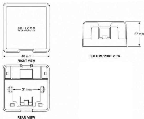
Bellcom 1-Port Surface Mount Box - Dimension Diagram
