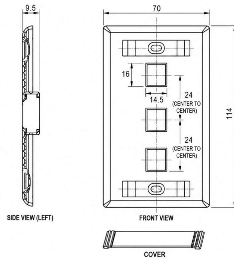
Bellcom 3-Port Window ID Keystone Faceplate
