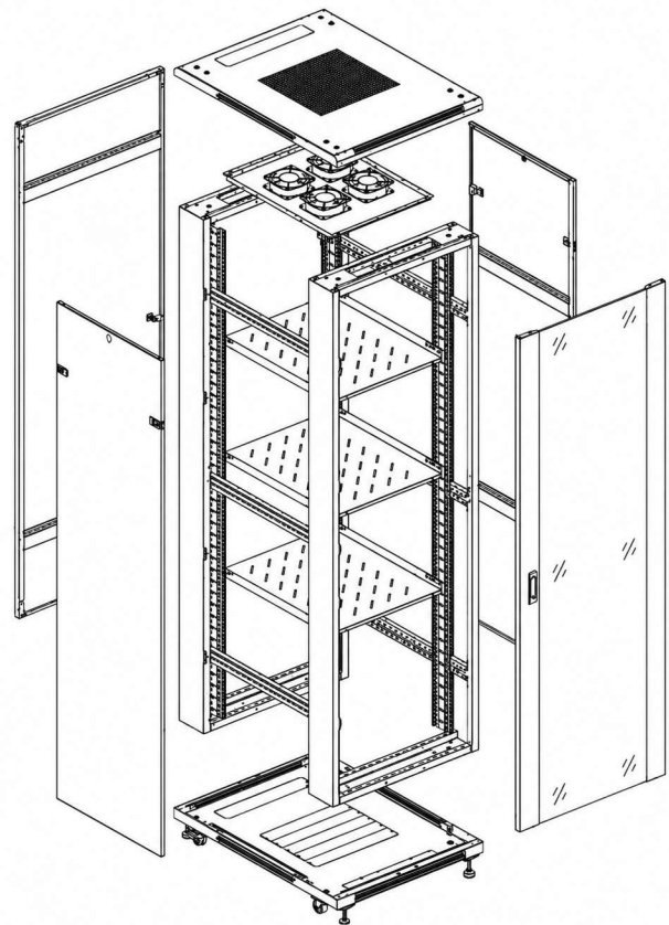
32U Network Cabinet
