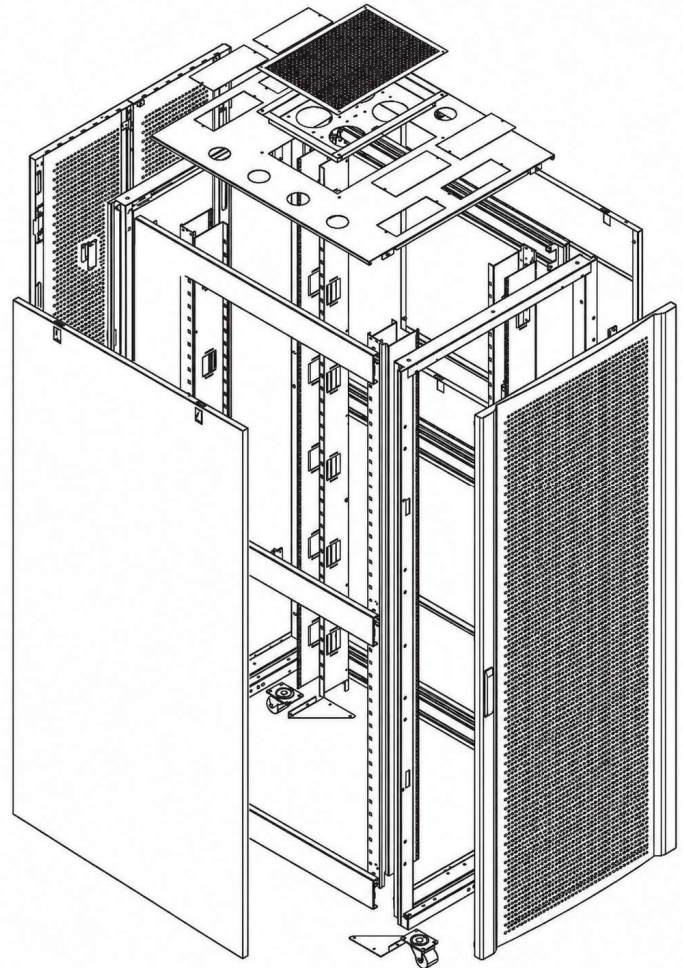
Bellcom 42U Server Cabinet
