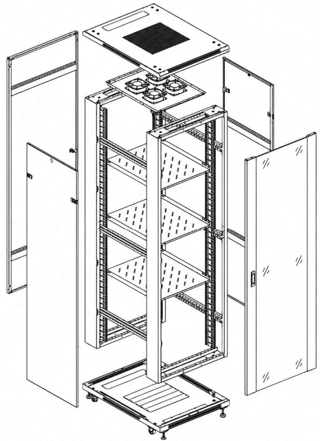
42U Network Cabinet
