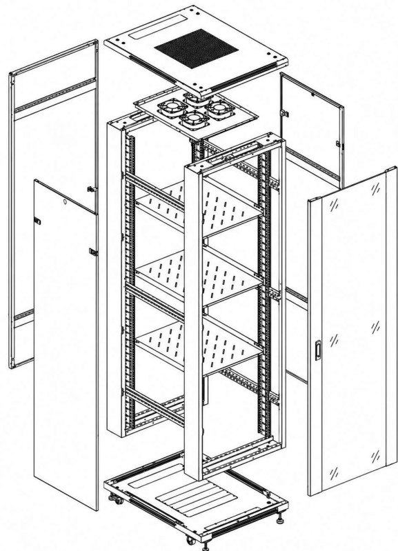
27U Network Cabinet
