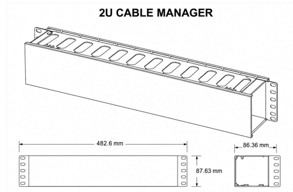
2U rack-mount cable manager with removable front cover
