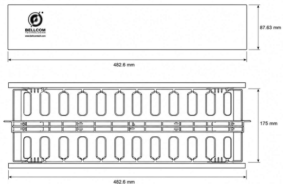
2U rack-mount double-sided cable manager
