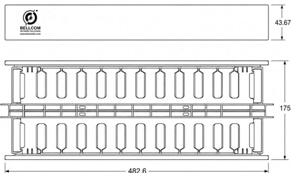
1U rack-mount double-sided cable manager
