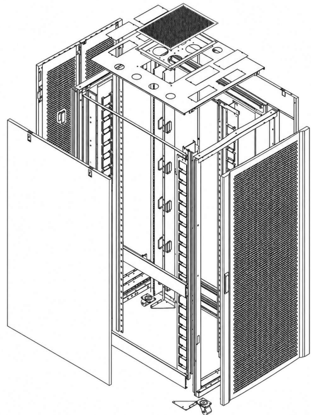
Bellcom 32U Server Cabinet
