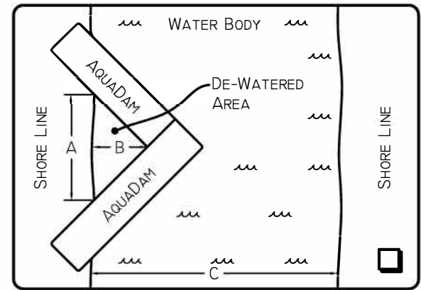
○ TP CONFIGURATION Scale: NTS
