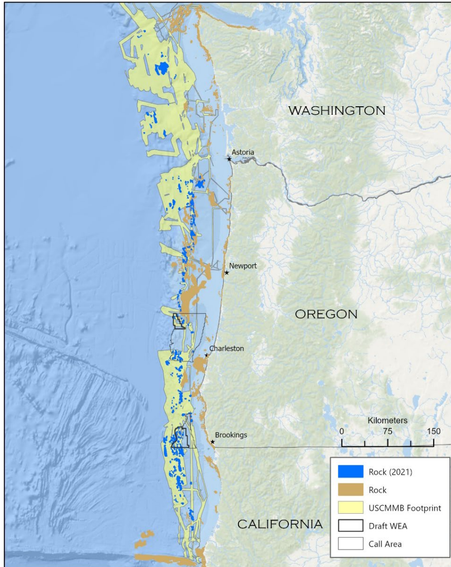
Figure 19: Map of methane-derived carbonate rock (blue polygons) on the Cascadia Margin identified by Merle et al (2021) in high-resolution multibeam backscatter data (yellow). Analysis limited to areas within the backscatter footprint that also coincide with water column bathymetry data. Backscatter data source: US Cascadia Margin Multibeam Backscatter (USCMMB)] (Merle, et al. 2021).
