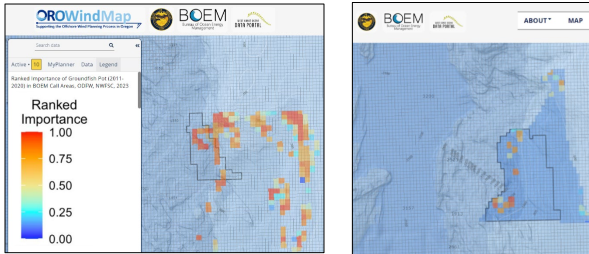
Figure 10: Groundfish pot ranked importance using ODFW and NWFS data. OROWindMap link: https://bit.ly/3RB1OAT . (left: Draft WEA A; right: Draft WEA B).
