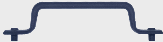
CH3826 L: 146mm H: 32mm C/C: 128mm
