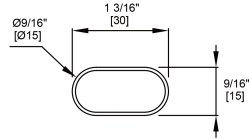
HORIZONTAL TUBE
