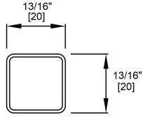
HORIZONTAL TUBE
