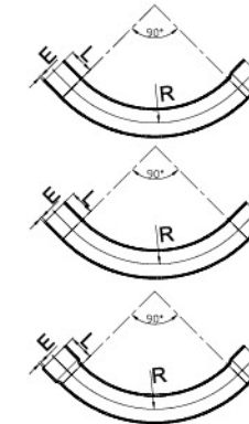
90° ELBOWS-one Bell END 90° ELBOWS-Plain END 90° ELBOW-Bell END
