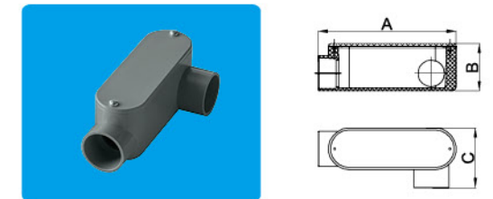
Conduit Bodies and covers Type LL
