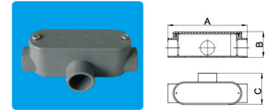
Conduit Bodies and covers Type T
