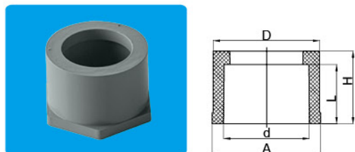
BUSHINGS
