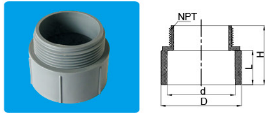
Male Adaptors
