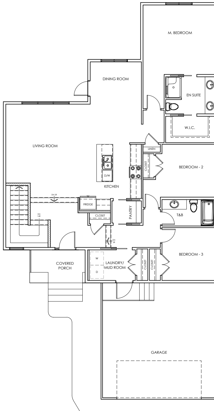
MAIN FLOOR PLAN (1642.0 SQ FT)
