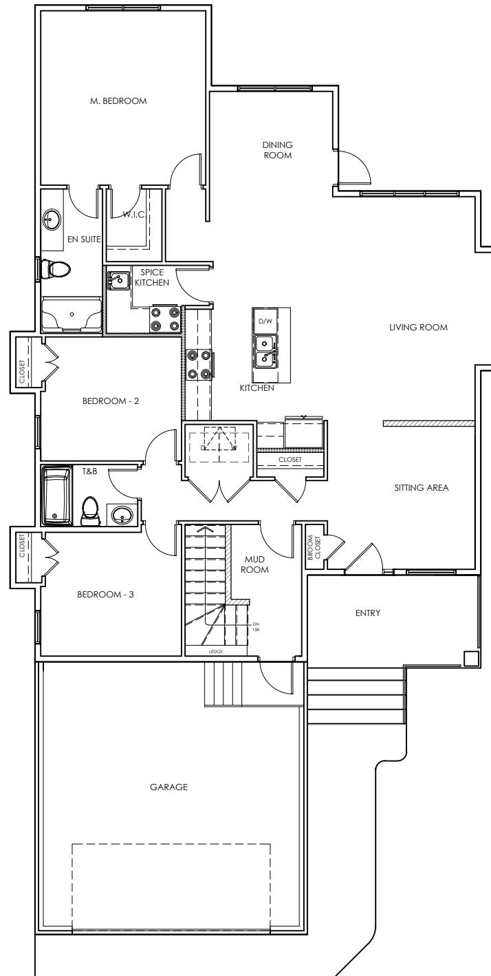
MAIN FLOOR PLAN (1605 SQ FT)
