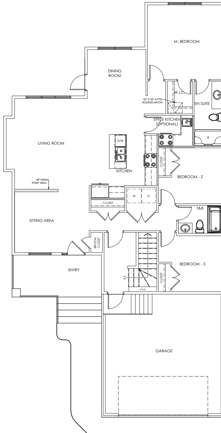
MAIN FLOOR PLAN (1585 SQ FT)
