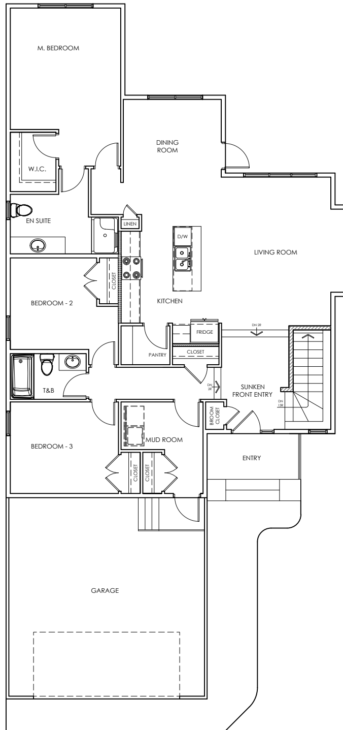
MAIN FLOOR PLAN (1529.0 SQ FT)
