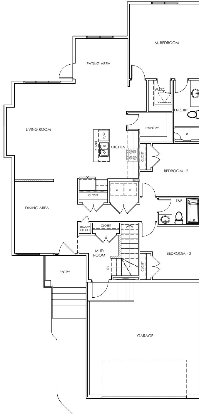
MAIN FLOOR PLAN (1614 SQ FT)
