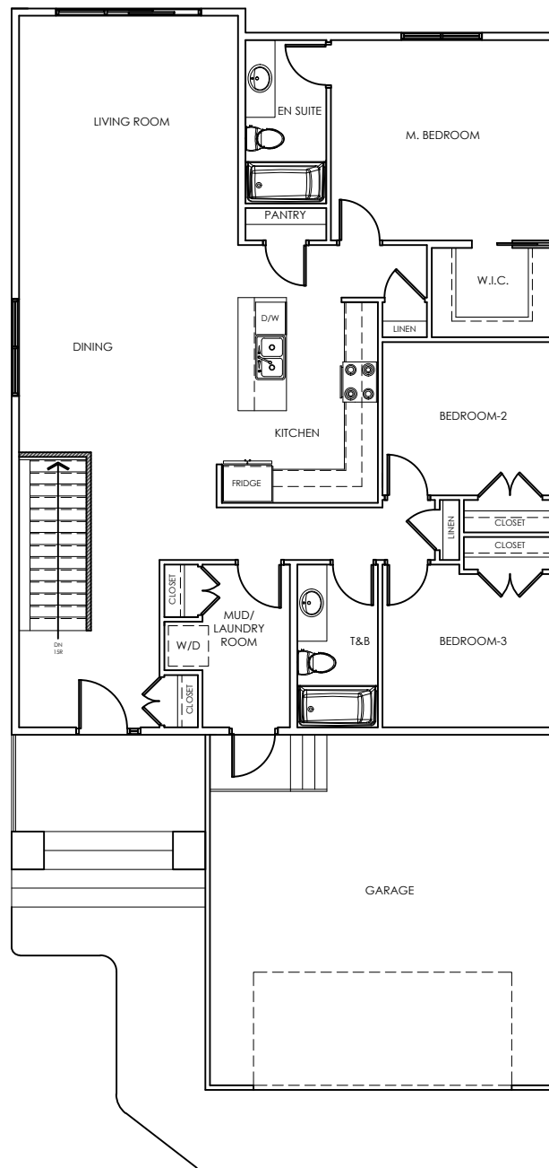
MAIN FLOOR PLAN (1500 SQ FT)
