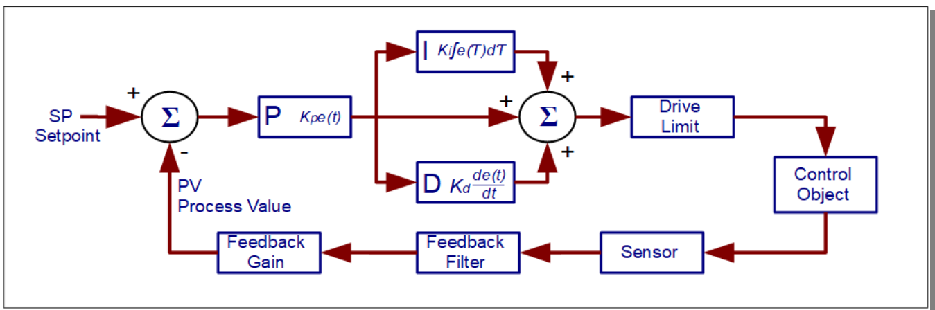
Graphic representation of the PID action.
