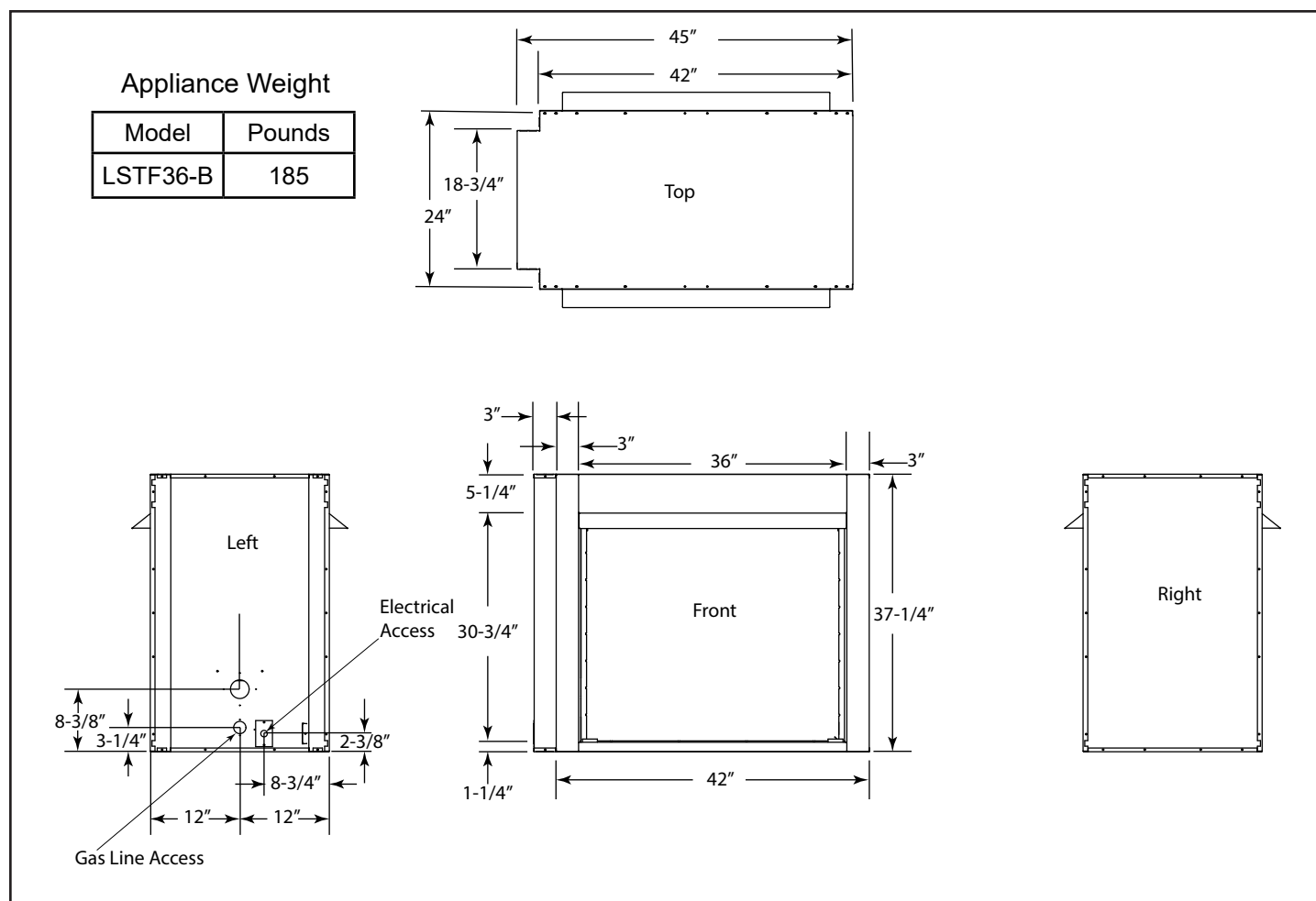
Figure 4.1 Framing Dimensions
