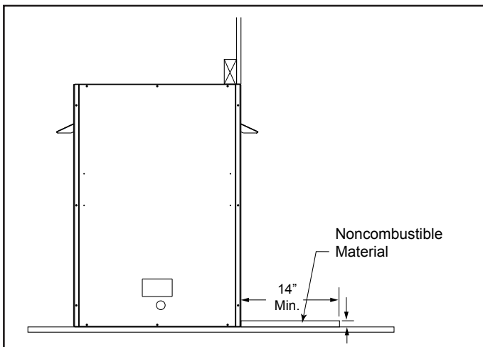
Figure 6.6 Floor Clearance Above Noncombustible Flooring Material
