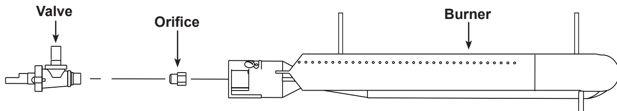
Fig. 32-1 - Main burner orifice diagram
