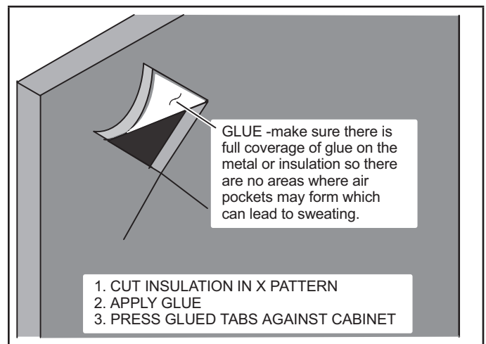
FIGURE 21. Repairing Insulation
