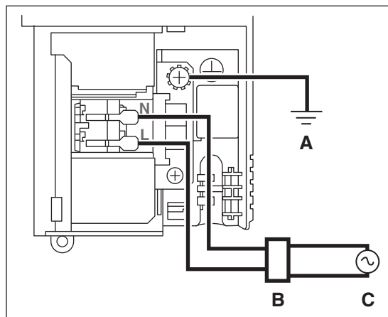
<Schematic power connection diagram>
