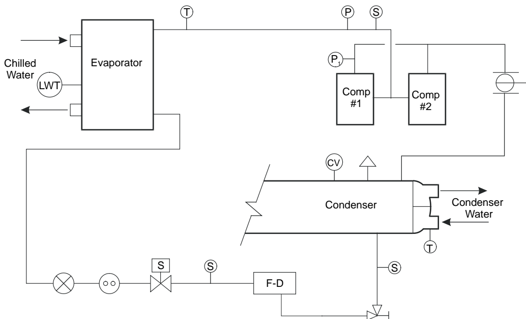
Figure 4, Schematic Piping Diagram (One of Two Circuits for WGZ030D – 130D)
