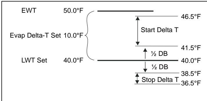
Figure 7, Staging/Starting Temperatures
