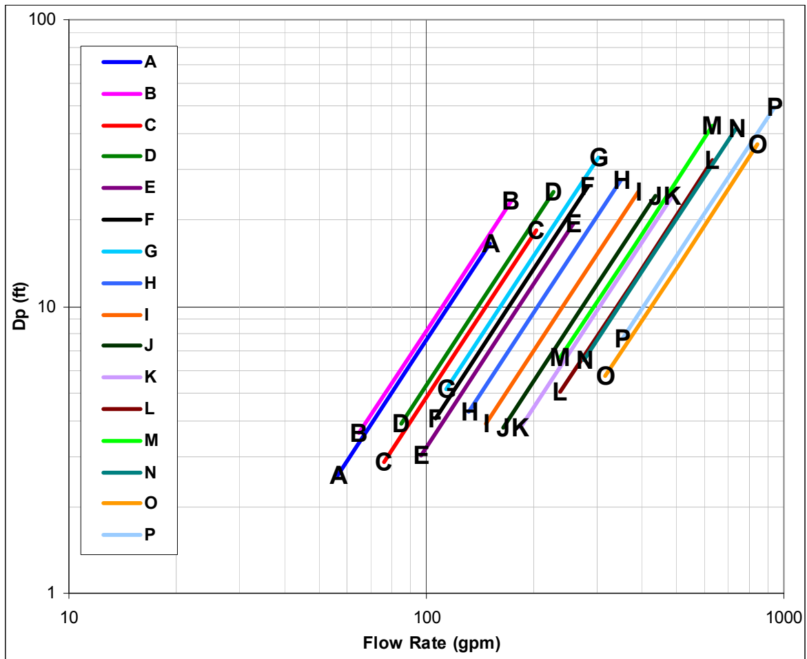
Figure 2, Condenser Pressure Drop, WGZ030D – WGZ200D
