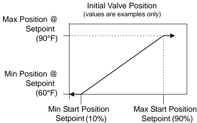
Figure 11, Initial Valve Position
