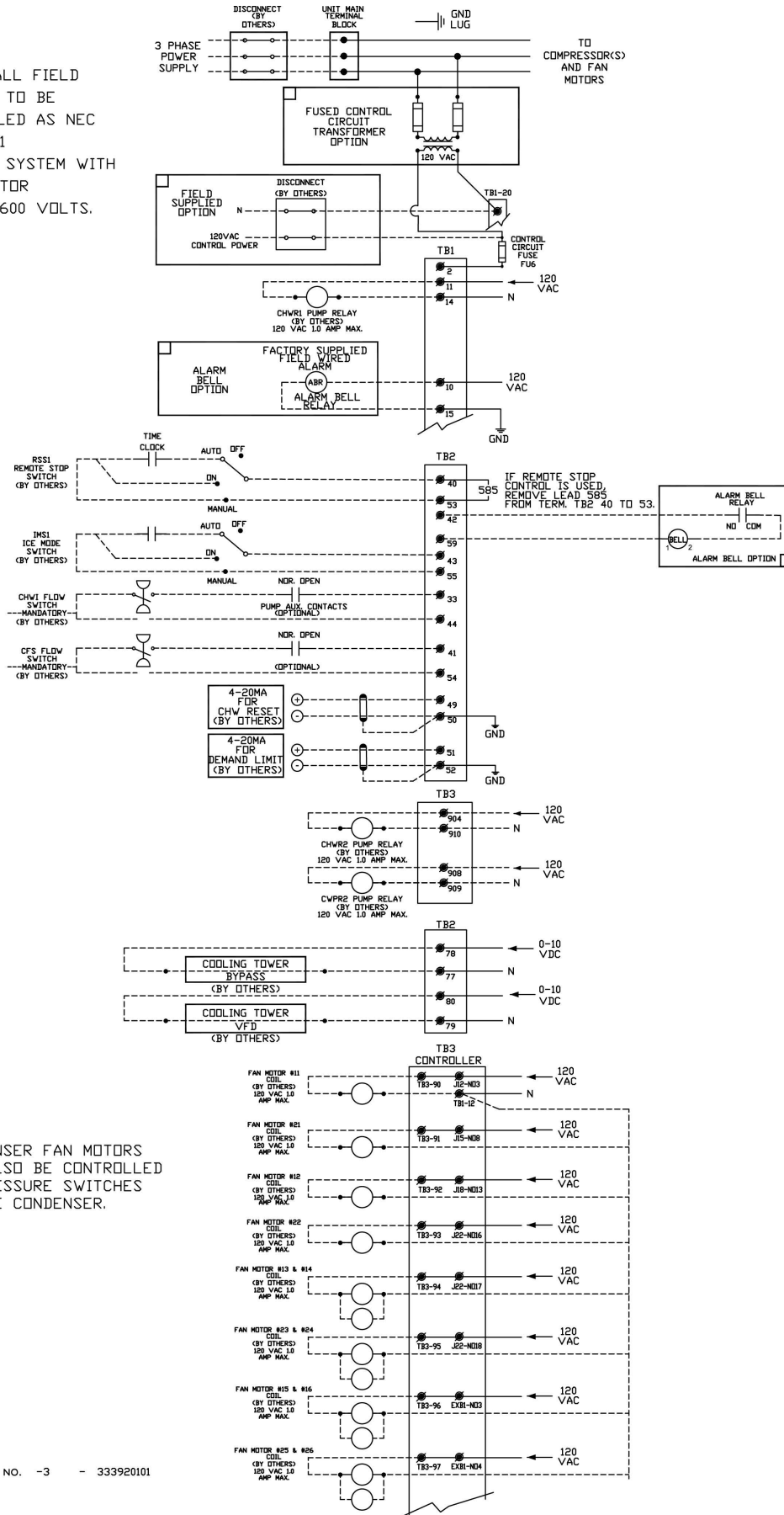
Figure 6, WGZ030DA – WGZ200DA Field Wiring Diagram (Remote Condenser)
