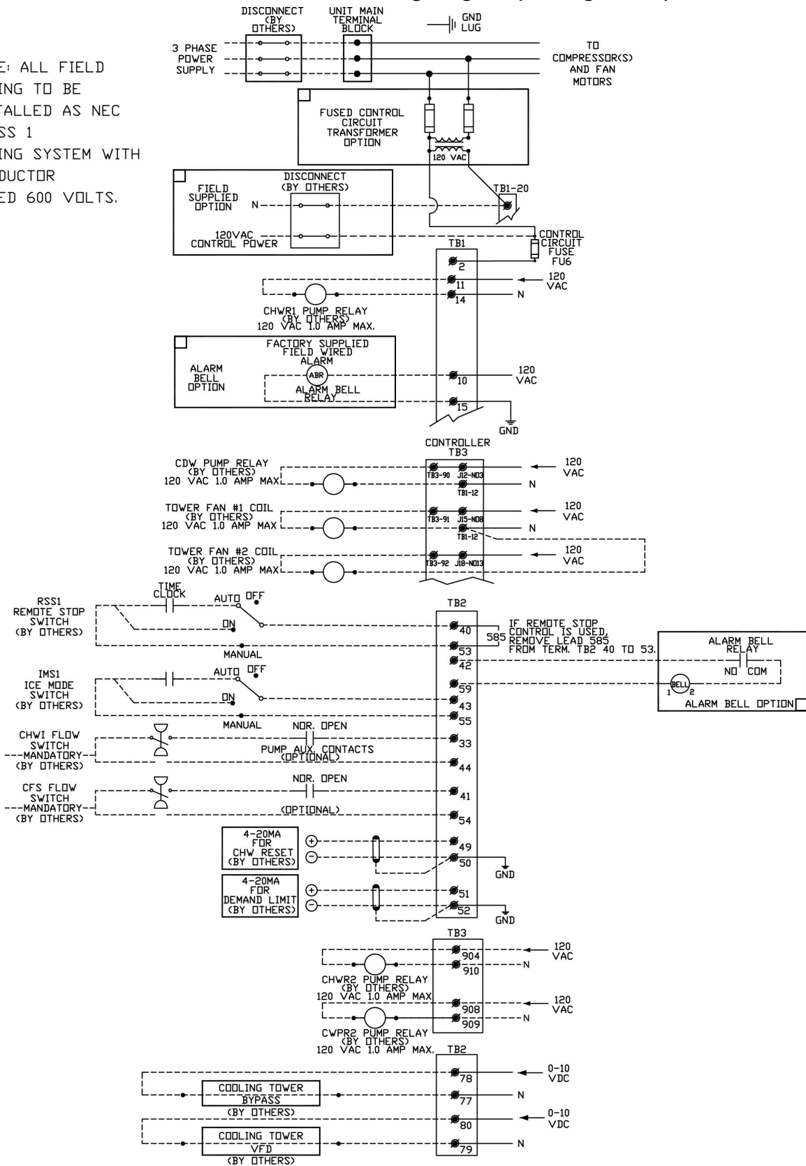
Figure 5, WGZ030DW – WGZ200DW Field Wiring Diagram (Packaged Unit)
