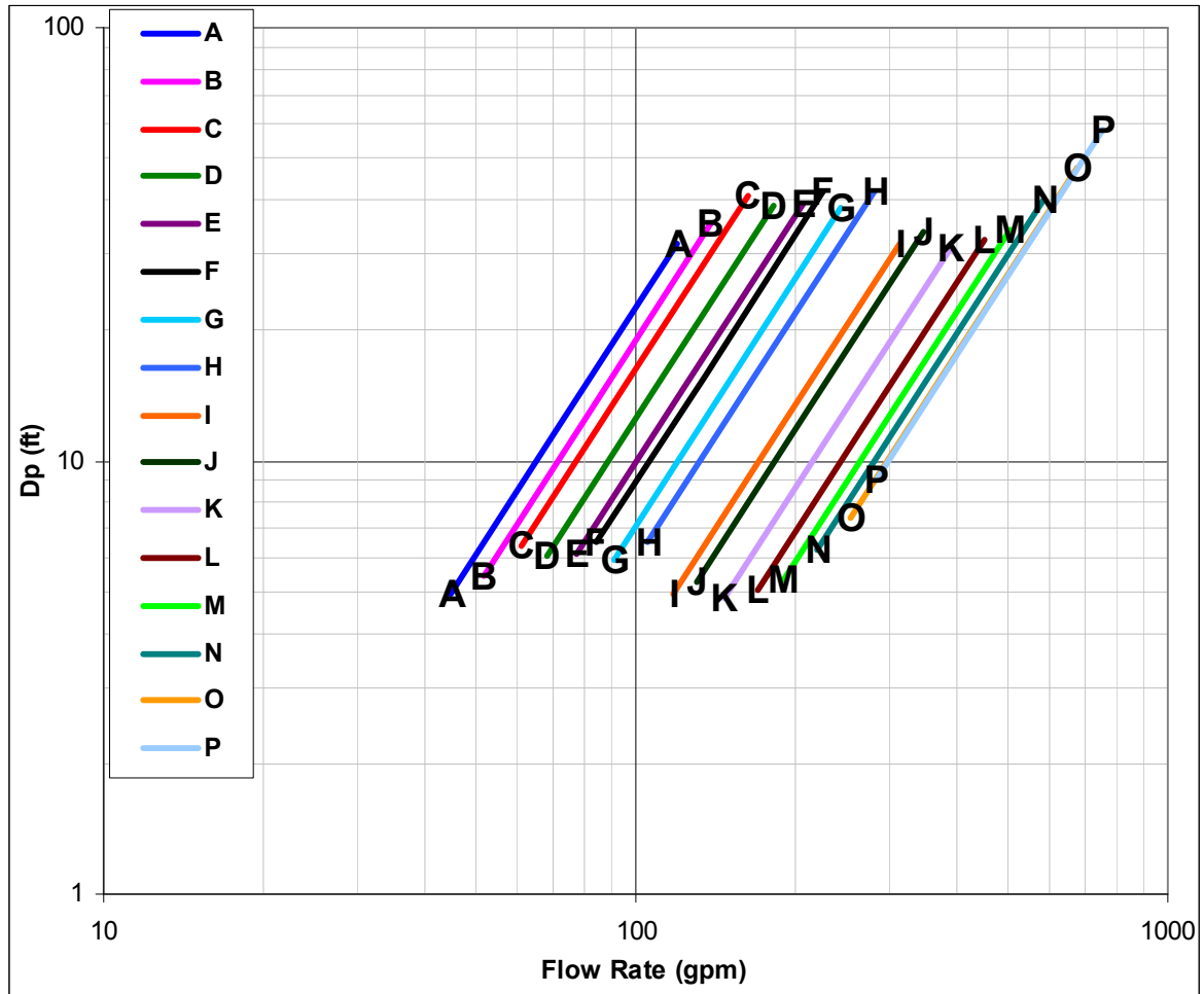
Figure 1, Evaporator Pressure Drop, WGZ030D – WGZ200D
