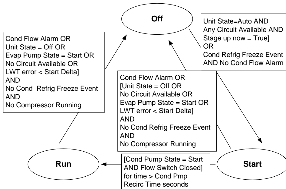
Condenser Pump State Diagram
