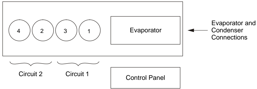
Figure 3, Compressor Locations
