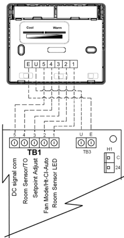
Figure 38: Adjustable Cool/Warm with Occupancy Switch – P/N 910121753
