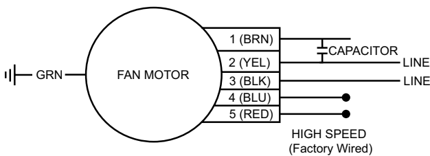
Figure 24: Size 042, 048, 060, 070 (380/50/3 and 460/60/3) factory wired for high speed
