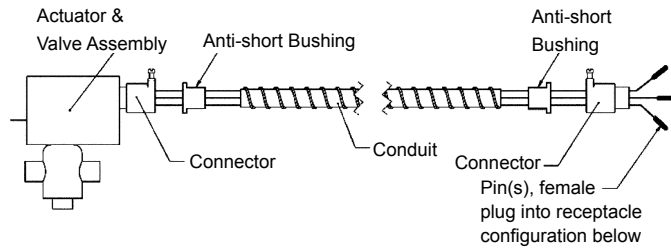
Figure 41: Normally Closed, Power Open Motorized Valve & Relay Wiring
