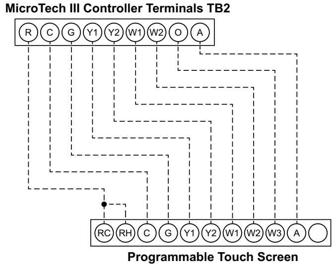
Figure 28: Programmable Electronic Thermostat 3 Heat/2 Cool, 7-Day Programmable, Auto Changeover, Hardwired – P/N 910193128 & Wi-Fi P/N 910193133
