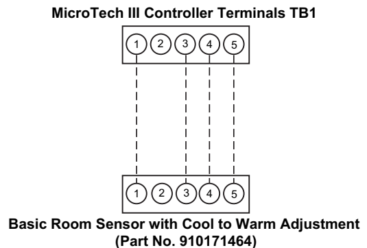
Figure 35: Cool/Warm Adjustable Sensor – P/N 910171464
