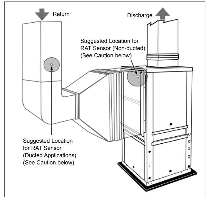
Figure 40: Return Air Temperature Sensor (RAT) locations
