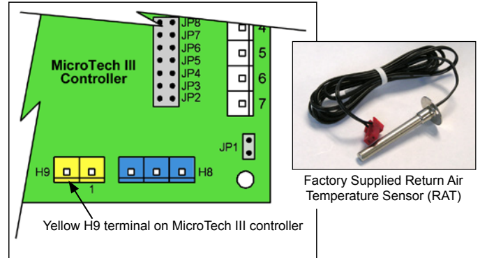
Figure 39: Units equipped with dehumidification and thermostat control. Factory supplied return air sensor connects to H9 terminal.
