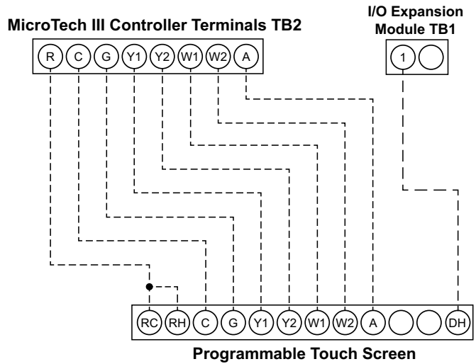
Figure 29: Programmable Electronic Thermostat 2 Heat/2 Cool, 7-Day Programmable, Dehumidification, Auto Changeover, Hardwired – P/N 910193129 & Wi-Fi P/N 910193134
