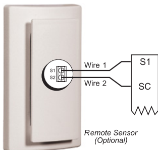
Figure 32: Remote Room Sensor Used With Thermostats 910193126, 910193127, 910193128, 910193129, 910193131, 910193132, 910193133, 910193134 – P/N 667720401
