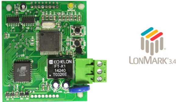
Figure 14: LONWORKS Communication Module
