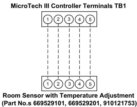
Figure 37: Room sensor with temperature adjustment wiring
