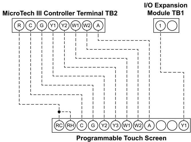
Figure 27: Programmable Electronic Thermostat 2 Heat/3 Cool, 7-Day Programmable, Auto Changeover, Hardwired – P/N 910193127 & Wi-Fi P/N 910193132
