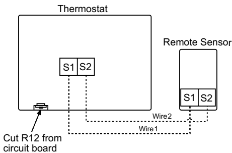
Figure 31: Remote Room Sensor Used With Thermostats 910121746 & 910121748 – P/N 107096010
