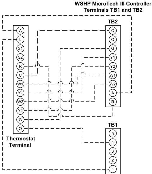
Figure 30: Programmable & Non-Programmable Electronic Thermostats 2 Heat/2 Cool, Auto Changeover, Hardwired – P/N 910121746 & P/N 910121748
