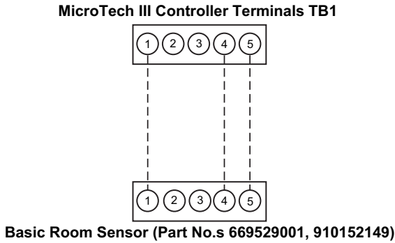
Figure 36: Basic sensor – P/N 910152149
