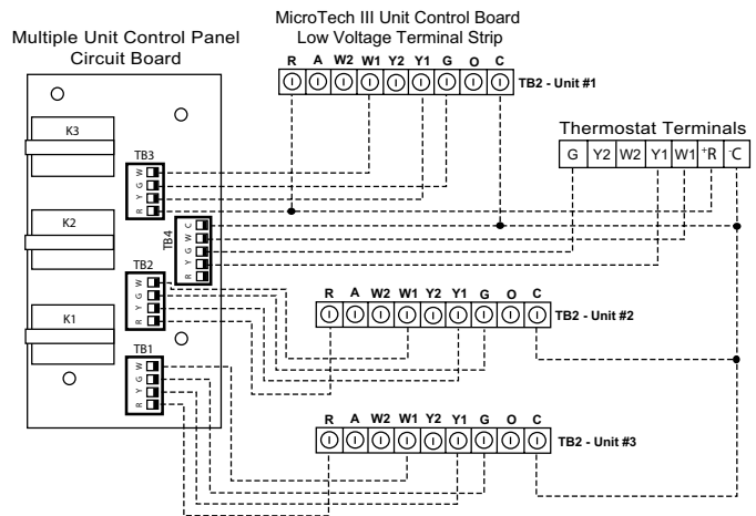
Figure 43: Wiring Multiple Unit Control Board (MUCP)
