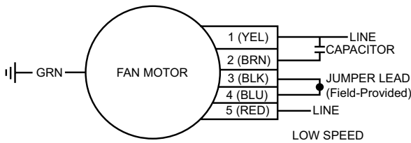
Figure 23: Size 042, 048, 060, 070 (575/60/3) low speed
