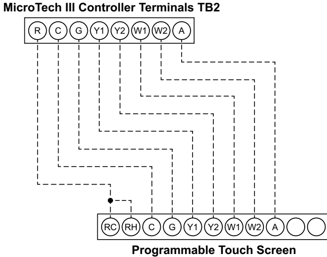
Figure 26: Programmable Electronic Thermostat 2 Heat/2 Cool, 7-Day Programmable, Auto Changeover, Hardwired – P/N 910193126 & Wi-Fi P/N 910193131
