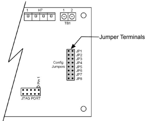
Figure 13: I/O Expansion Module Configuration Jumper Terminals
