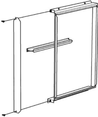
Figure 4: Sizes 007 thru 070 Optional 2" Return Air Duct Collar Filter Rack
