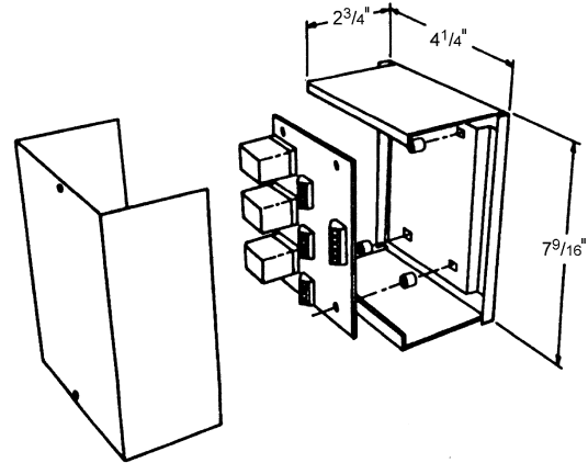
Figure 42: Multiple Unit Control Panel and Board
