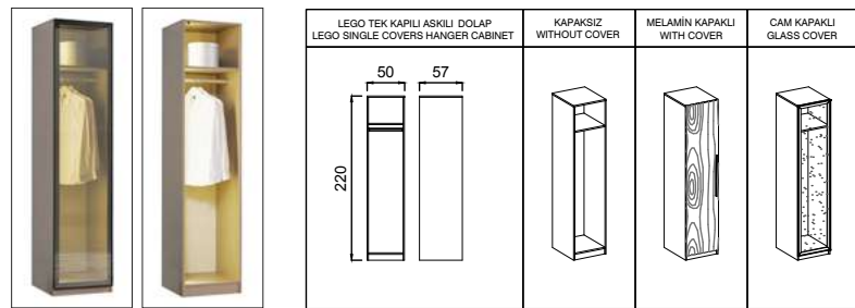
LEGO SINGLE COVERS HANGER CABINET
