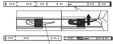
Trigger Disconnect Lever
